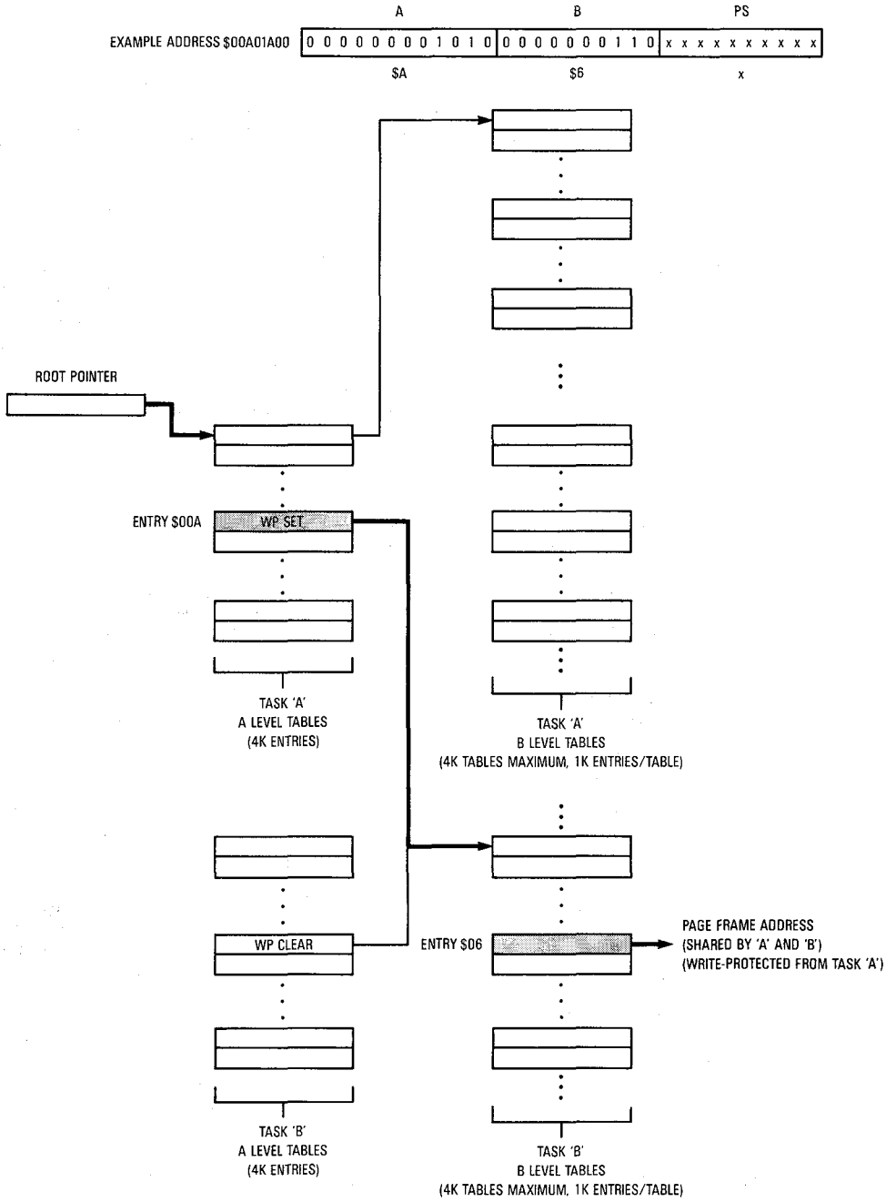
Figure 9-23. Example Translation Tree Using Shared Tables
