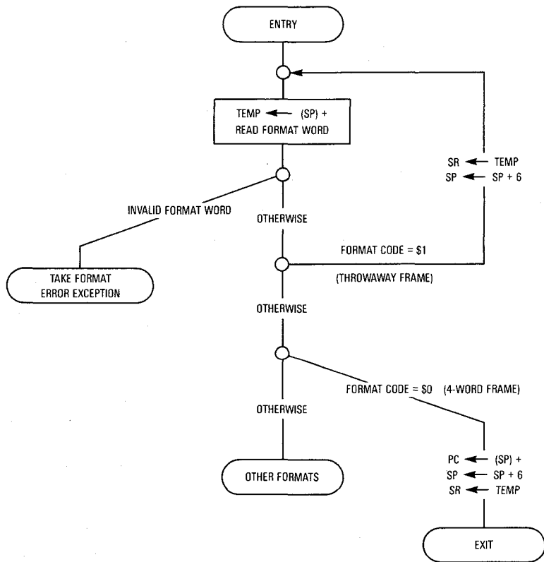
Figure 8-8. RTE Instruction for Throwing a Four-Word Frame
