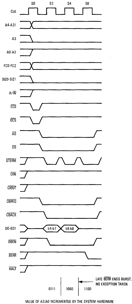
Figure 7-52. Long-Word Operand Request — Late BERR on Third Access
