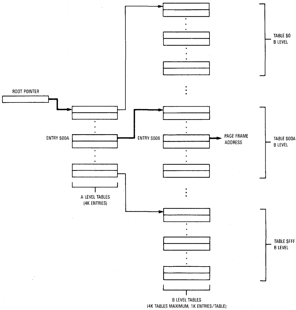
Figure 9-4. Example Translation Table Tree
