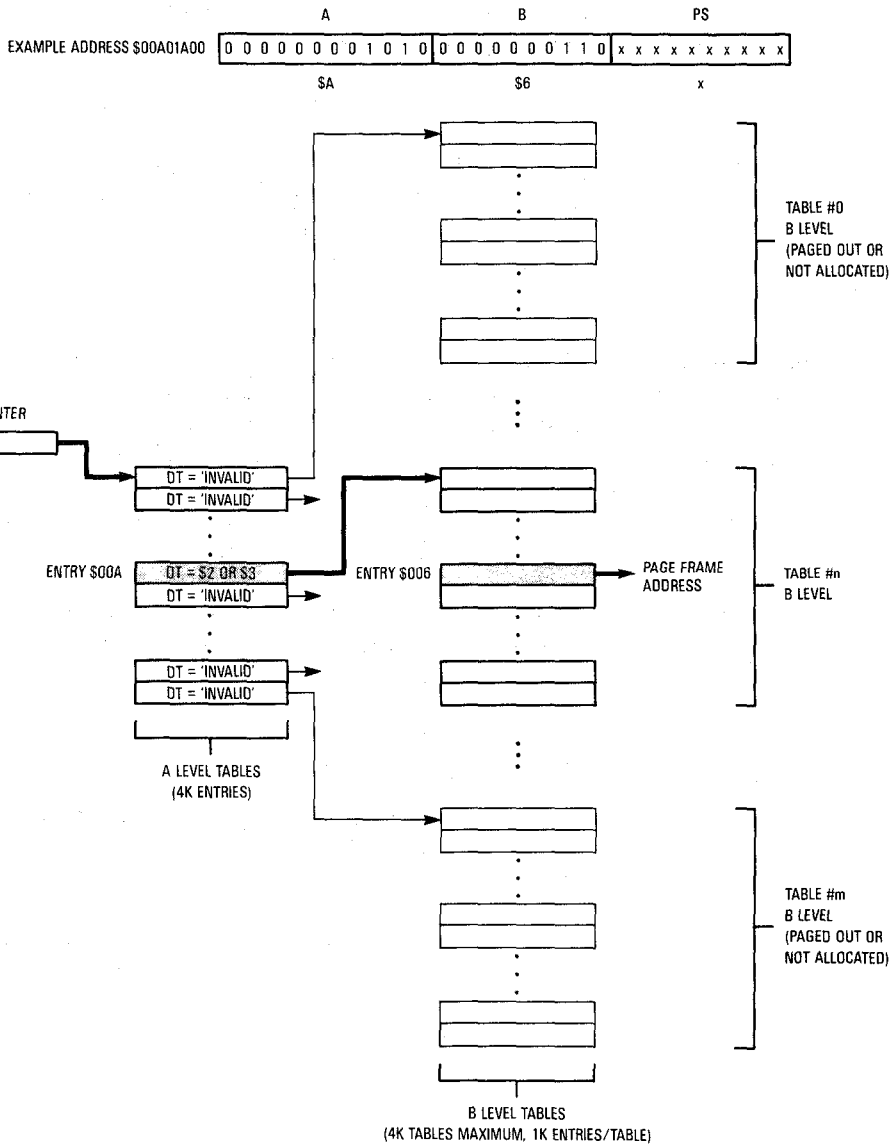
Figure 9-24. Example Translation Tree with Nonresident Tables
