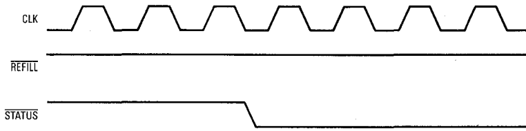
Figure 12-22. Processor Halted
