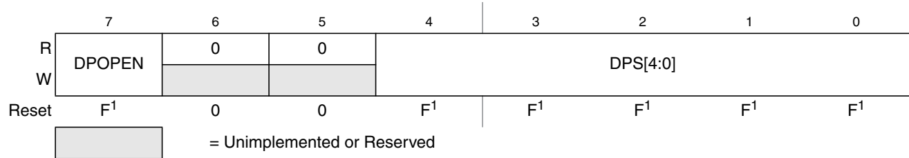
Figure 24-14. EEPROM Protection Register (EPROT)
